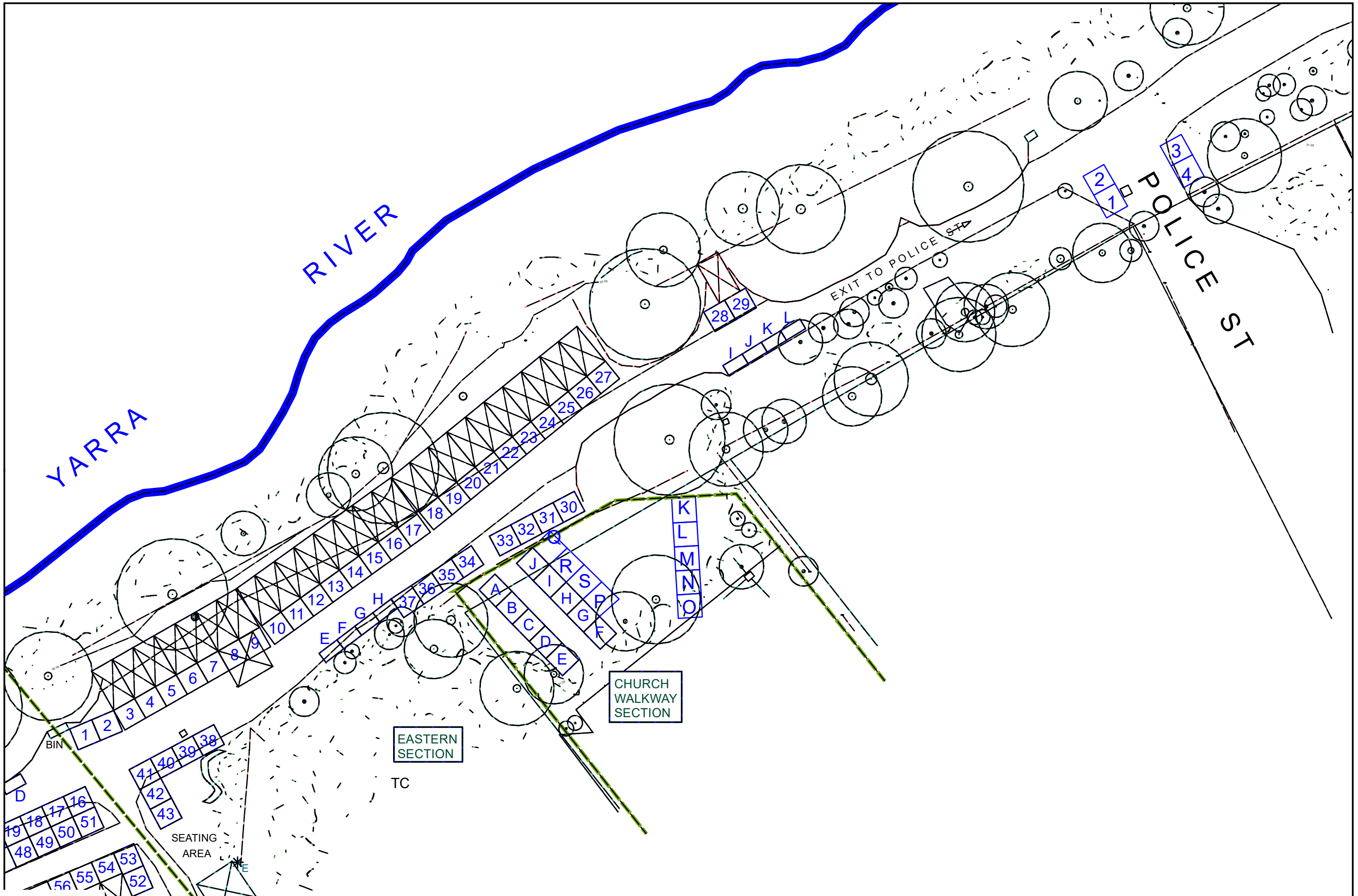
Warrandyte River Reserve - Warrandyte Riverside Market Stall Location Plan: Eastern Section + Church Walkway Section + Police Street Section
